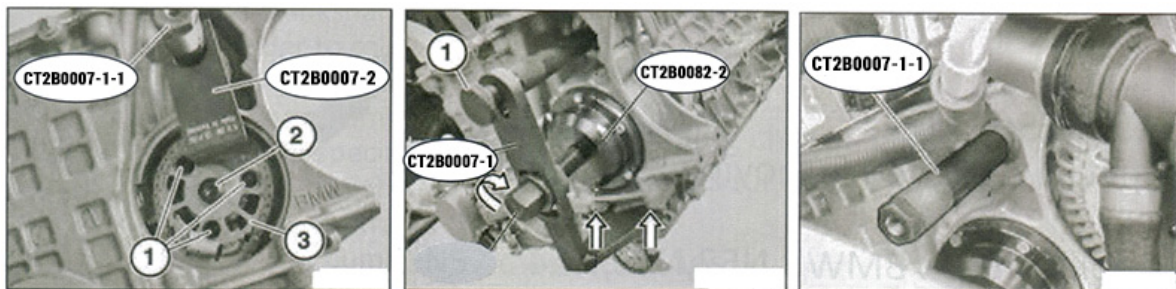
BMW N51 N52 Vacuum Pump Seal Cap Installer and Remover
